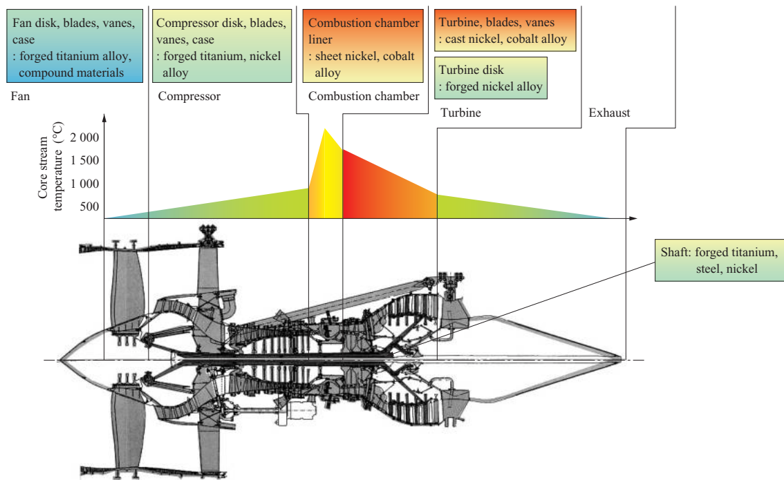
Schematic of jet engine
