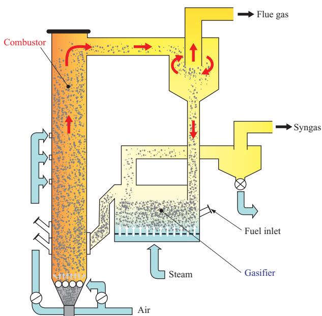
Structure and principle of the Twin IHI Gasifier (TIGAR®)
