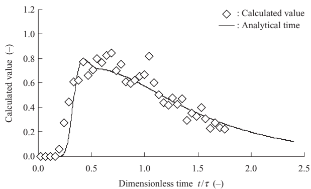
Fig. 6 RTD of coal particles (length: 3 m)
