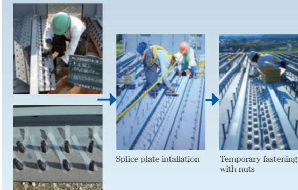
IS clip installation
