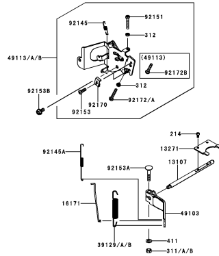
B-09 CONTROL-EQUIPMENT
