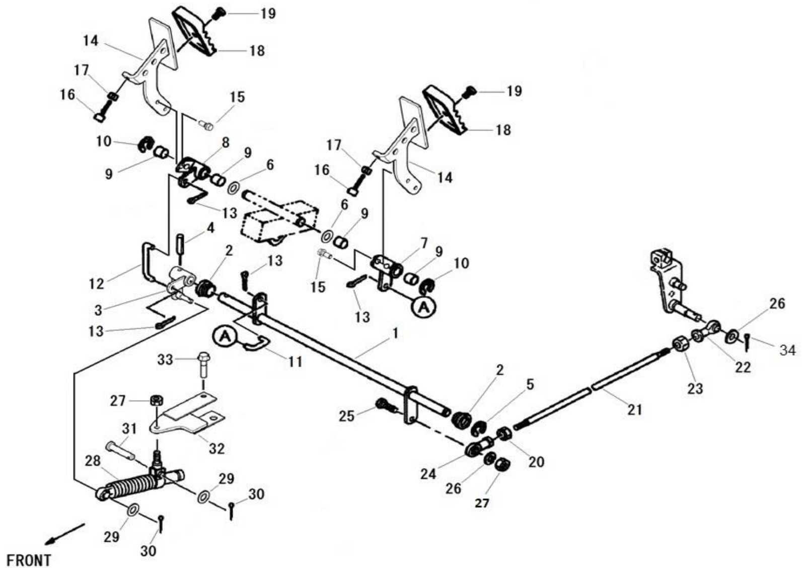
FIG.213 PEDALS, HYDROSTATIC TRANSMISSION H. S. Tペダル
