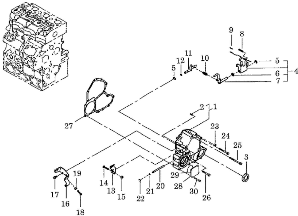
FIG.109 タイミングギヤ、ガバナ TIMING GEAR, GOVERNOR
