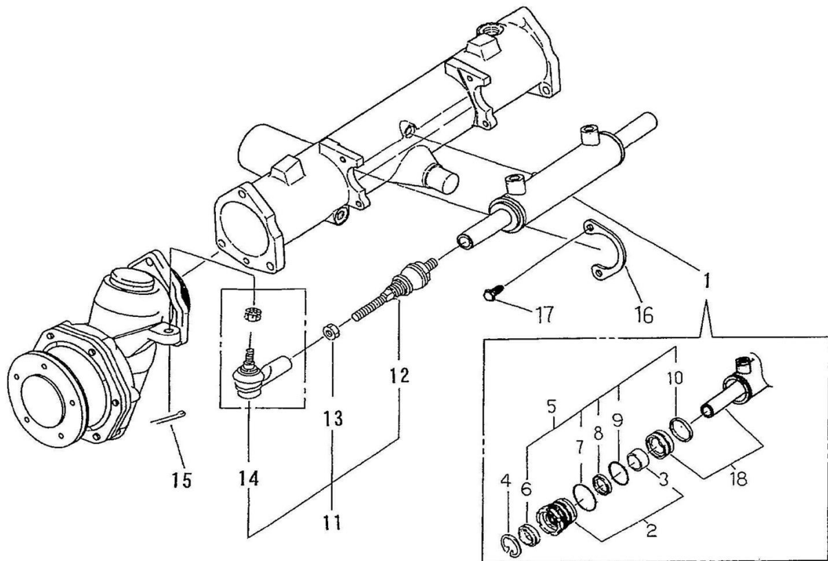
FIG.202 油圧シリンダ HYDROSTATIC CYLINDER
