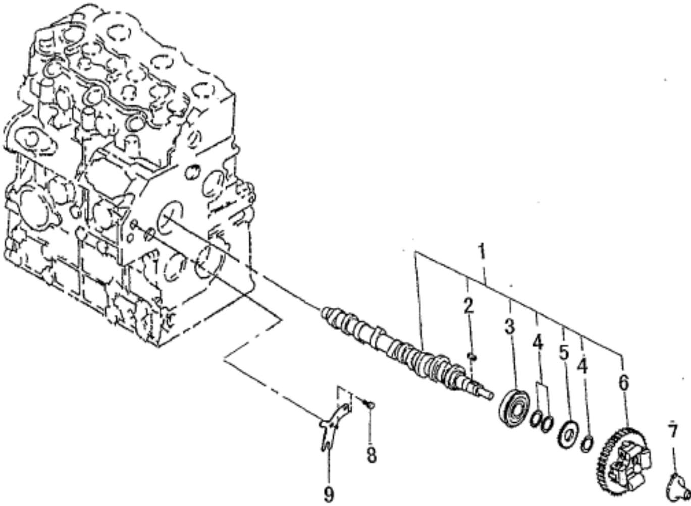
FIG.116 CAM SHAFT : MC284
