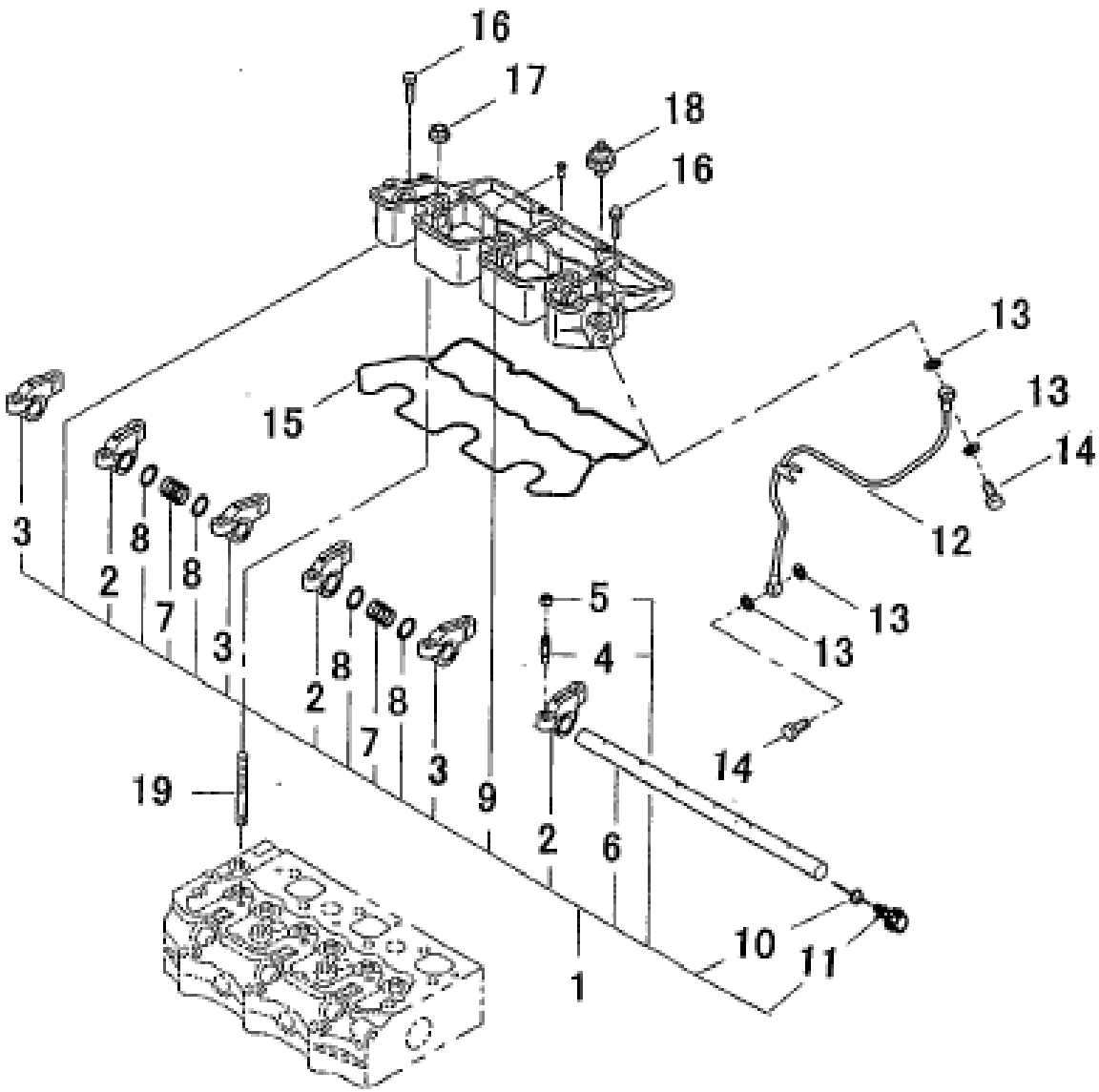
FIG.108 ROCKER ARM MC234 :TIRE 2
