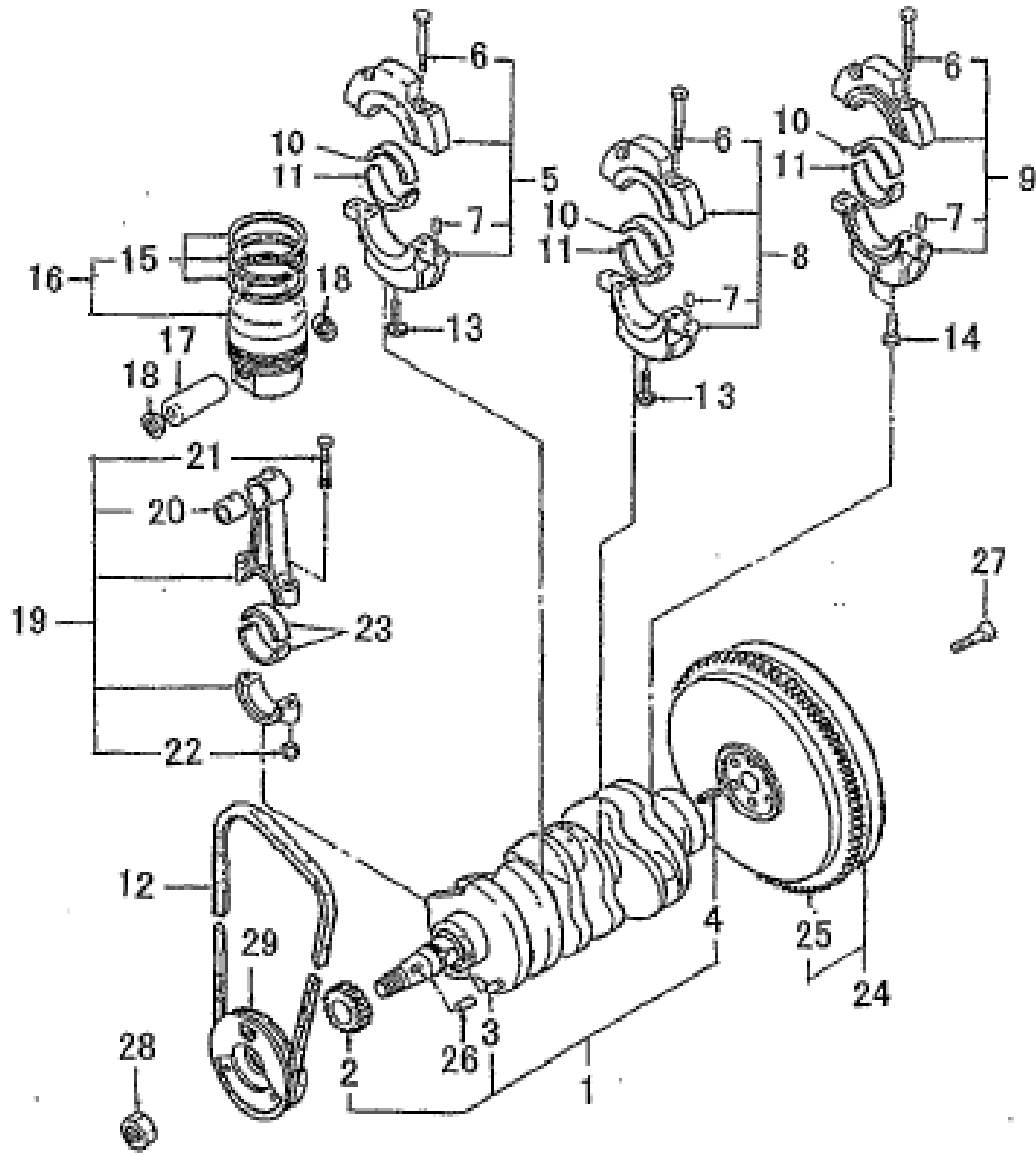
FIG.111 CRANK SHAFT , PISTON : MC234
