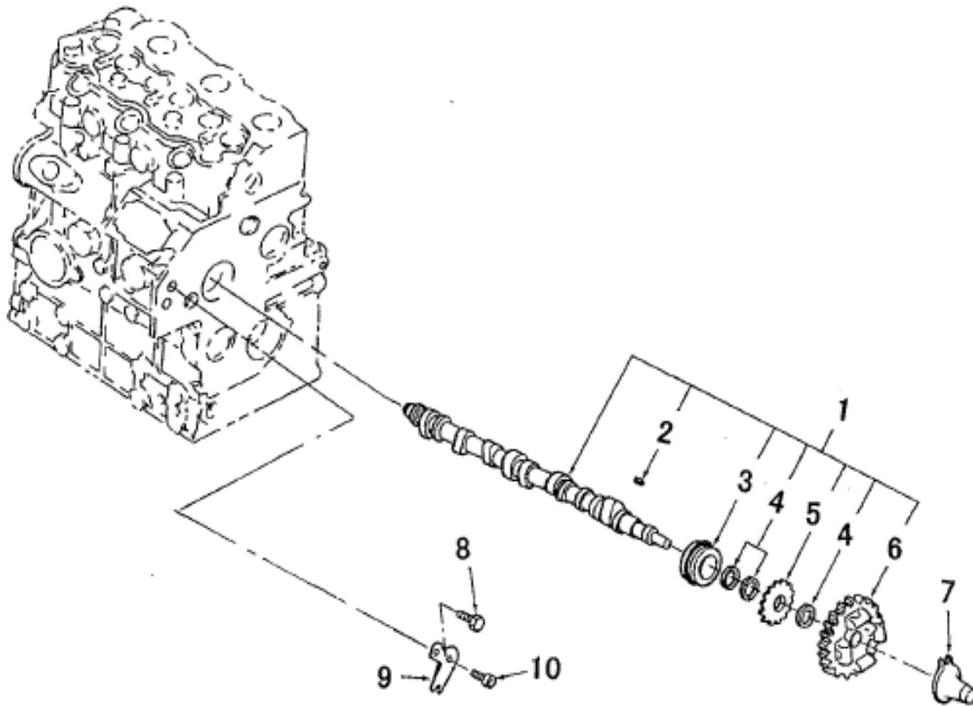
FIG.115 CAM SHAFT : MC234
