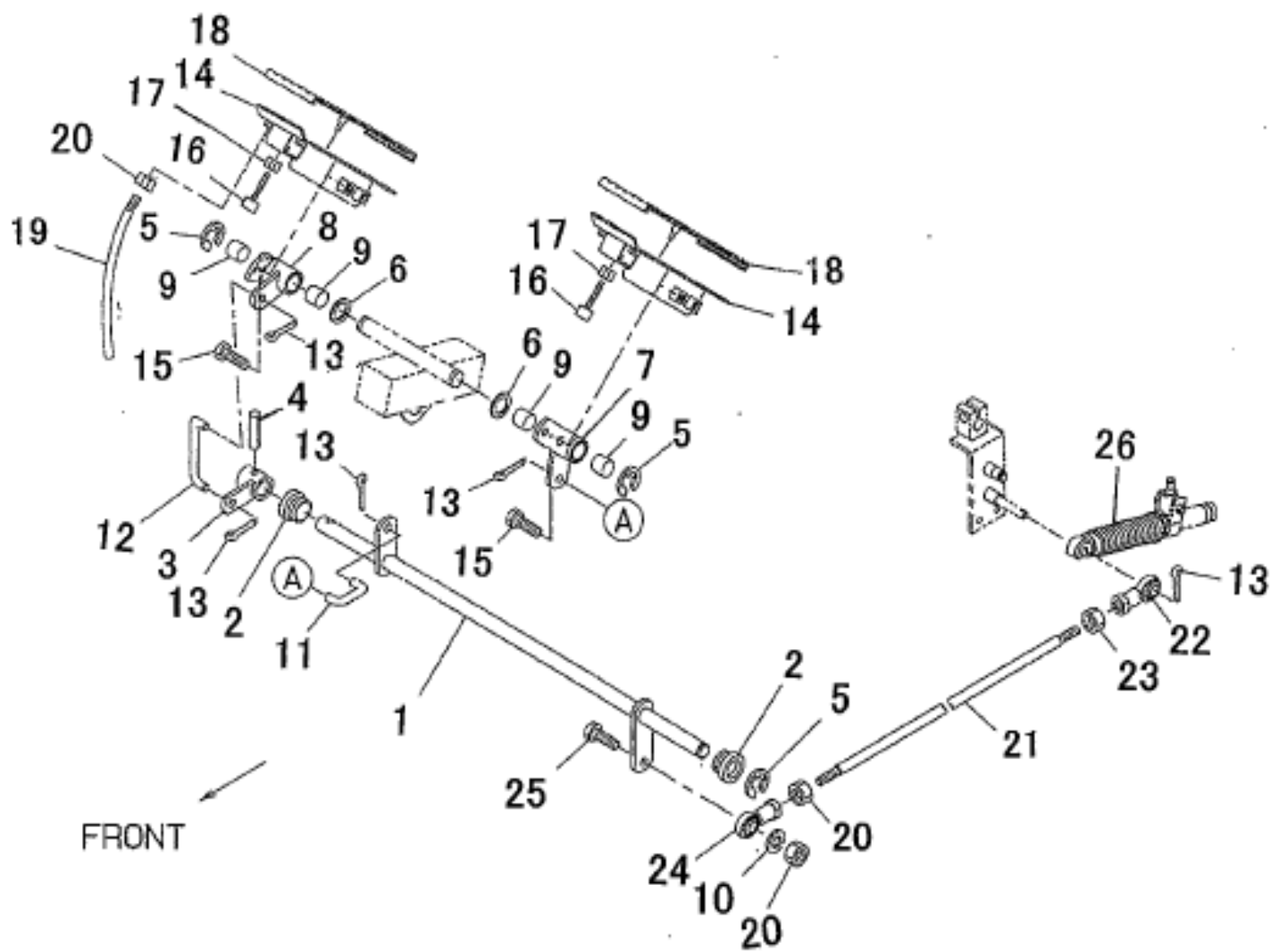
ペダル , HST FIG.215 PEDALS , HYDROSTATIC TRANSMISSION
