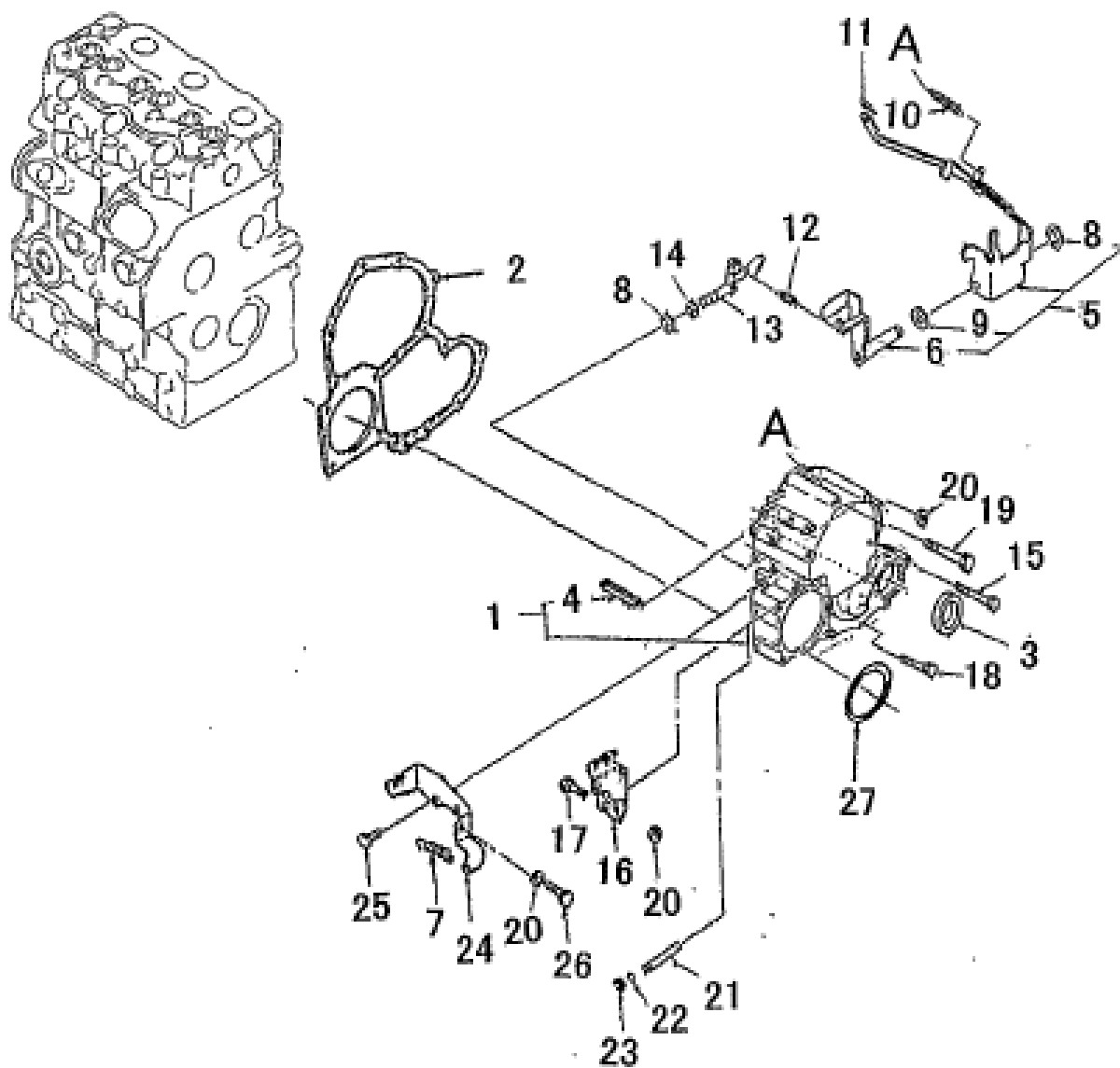
FIG.121 TIMING GEAR CASE, GOVERNOR : MC354
