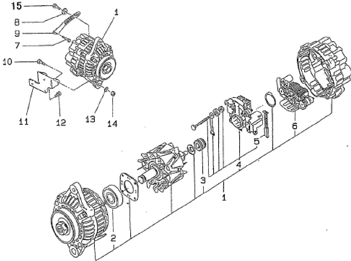
FIG.133 ALTERNATOR & MOUNTING :MC284/MC354
