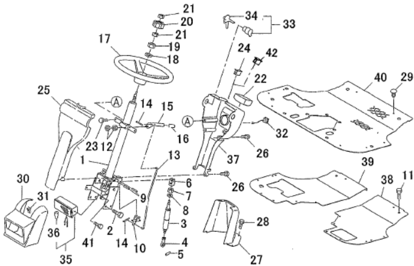
FIG.210 STEERING COLUMN &amp; STEP
