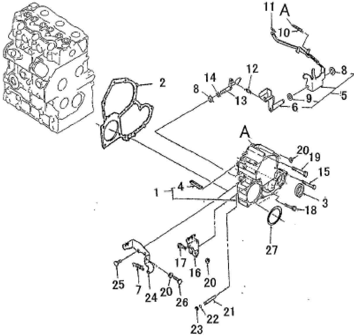
FIG.119 TIMING GEAR CASE, GOVERNOR : MC234
