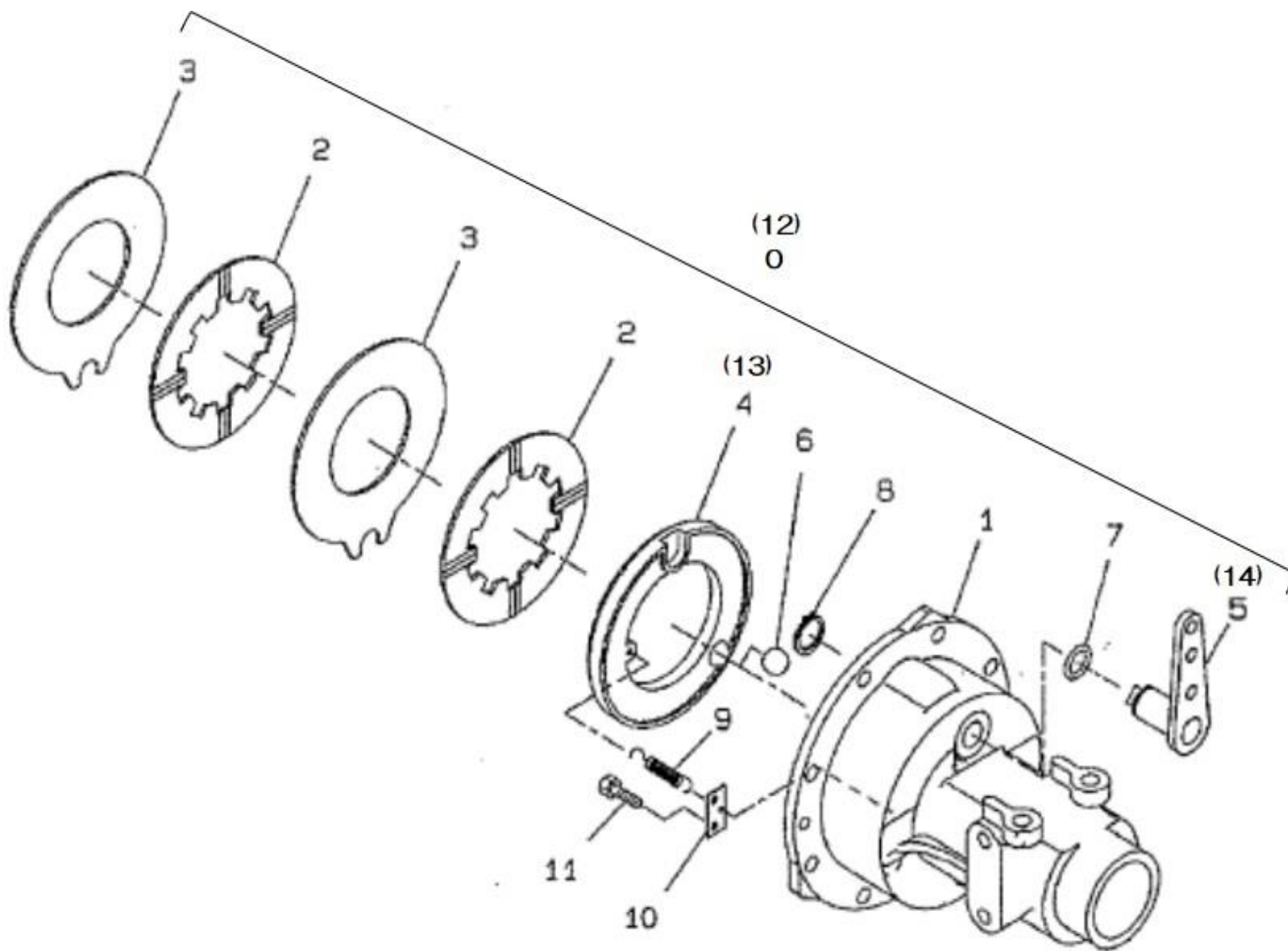
FIG.209 BRAKE ASSEMBLY
