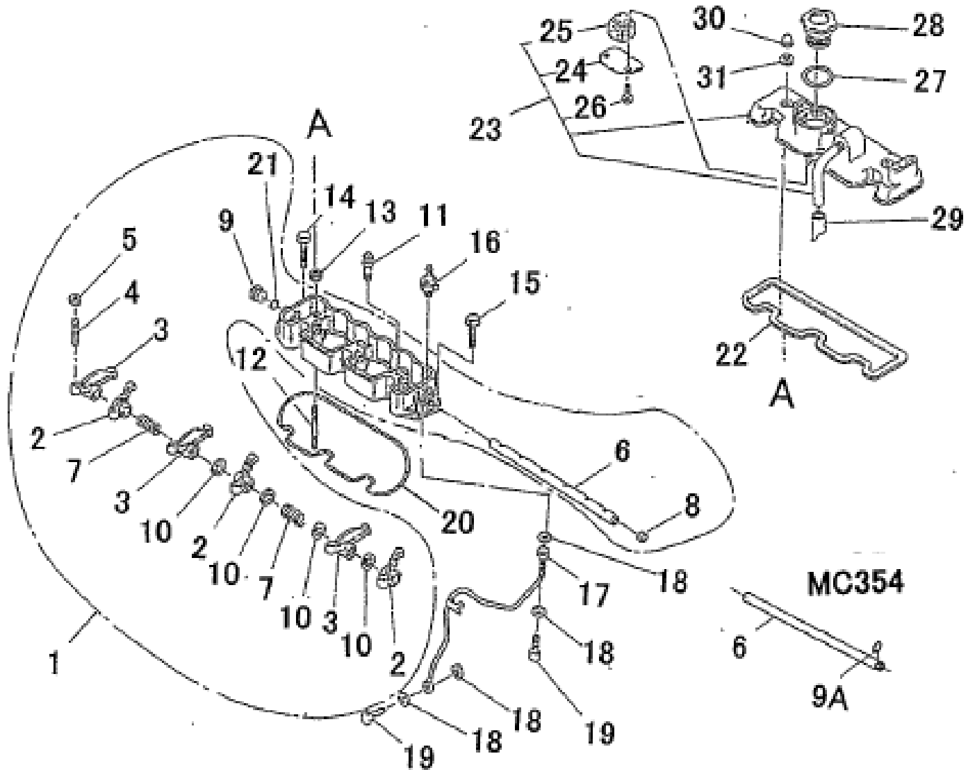
FIG.107 ROCKER ARM, HEAD COVER :TIRE 1
