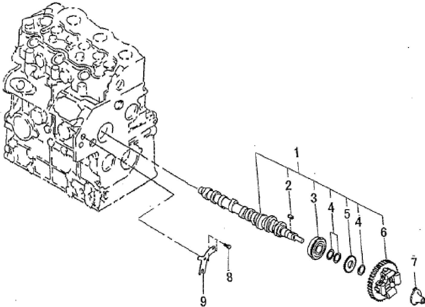
FIG.117 CAM SHAFT : MC354
