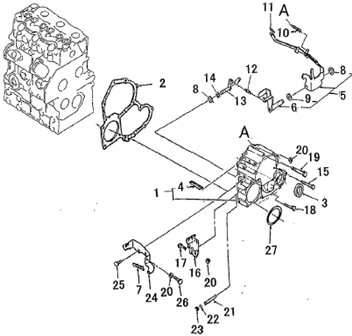
FIG.120 TIMING GEAR CASE, GOVERNOR : MC284
