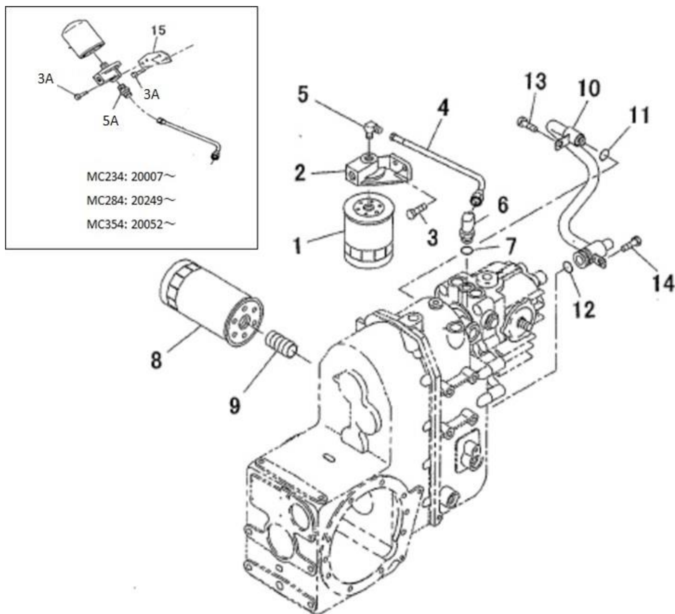
油圧フィルタ FIG.223 OIL FILTER ,HYDRAULICS
