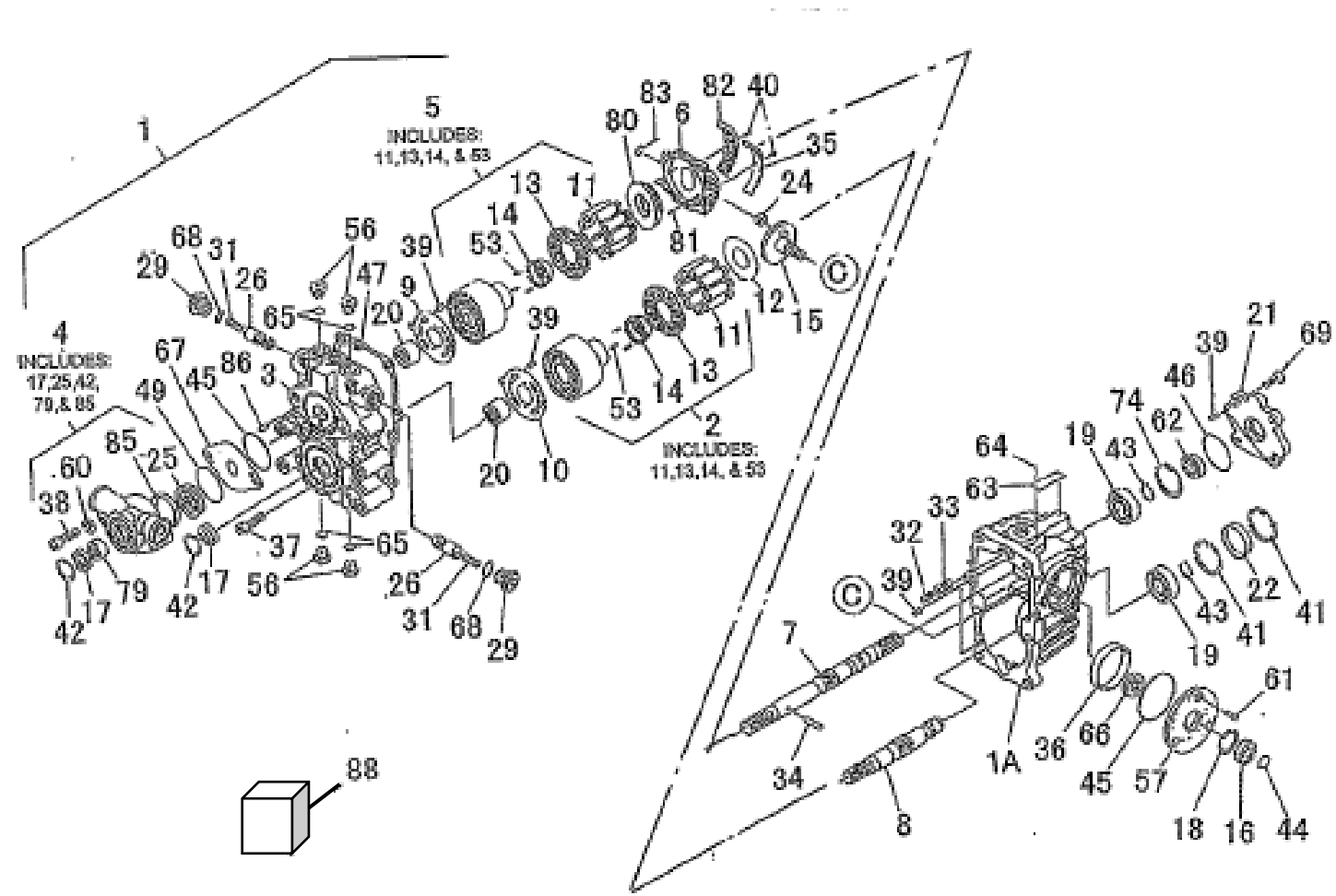
HST ASSY FIG.225 HYDROSTATIC TRANSMISSION ASSEMBLY
