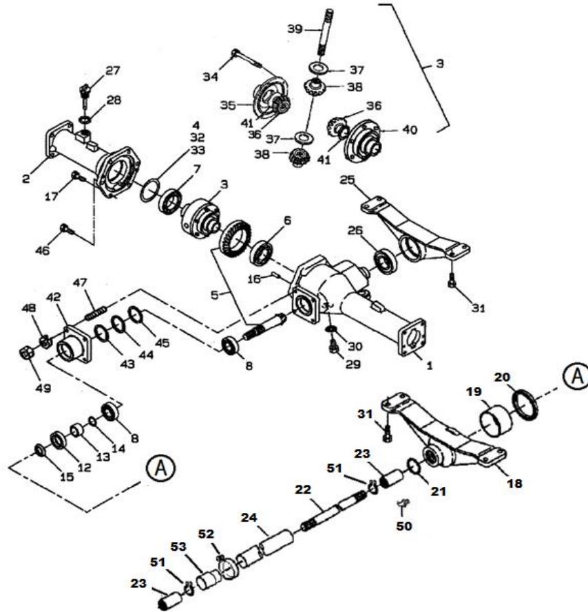
FIG.211 REAR AXLE , DIFFERNTIAL & HOUSING リヤアクスル, デフ&ハウジング
