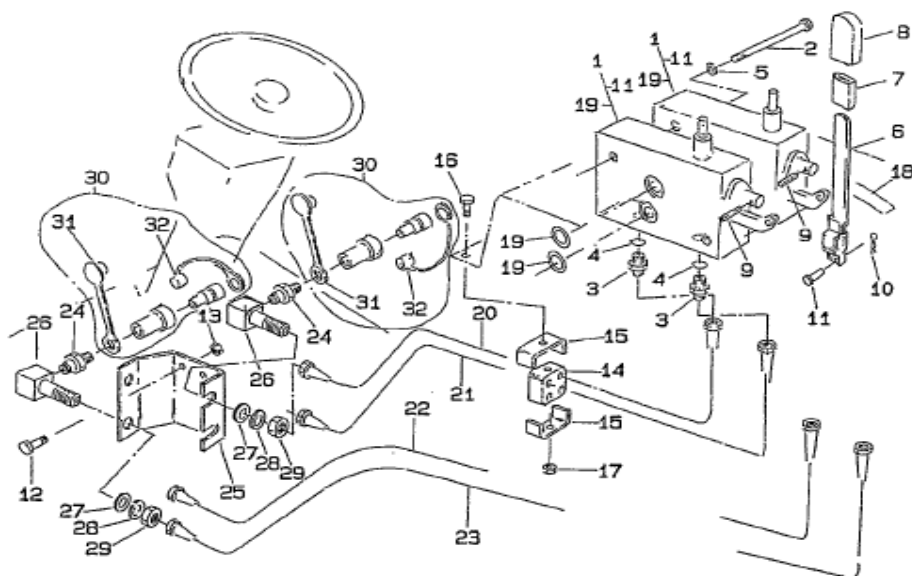
FIG.233 DUAL REMOTE HYD-VALVE (OPTION) サブバルブ:2連 (オプション)
