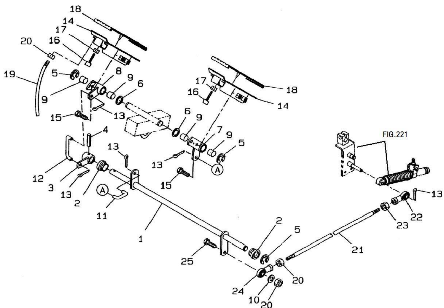
ペダル、HST FIG.213 PEDALS, HYDROSTATIC TRANSMISSION
