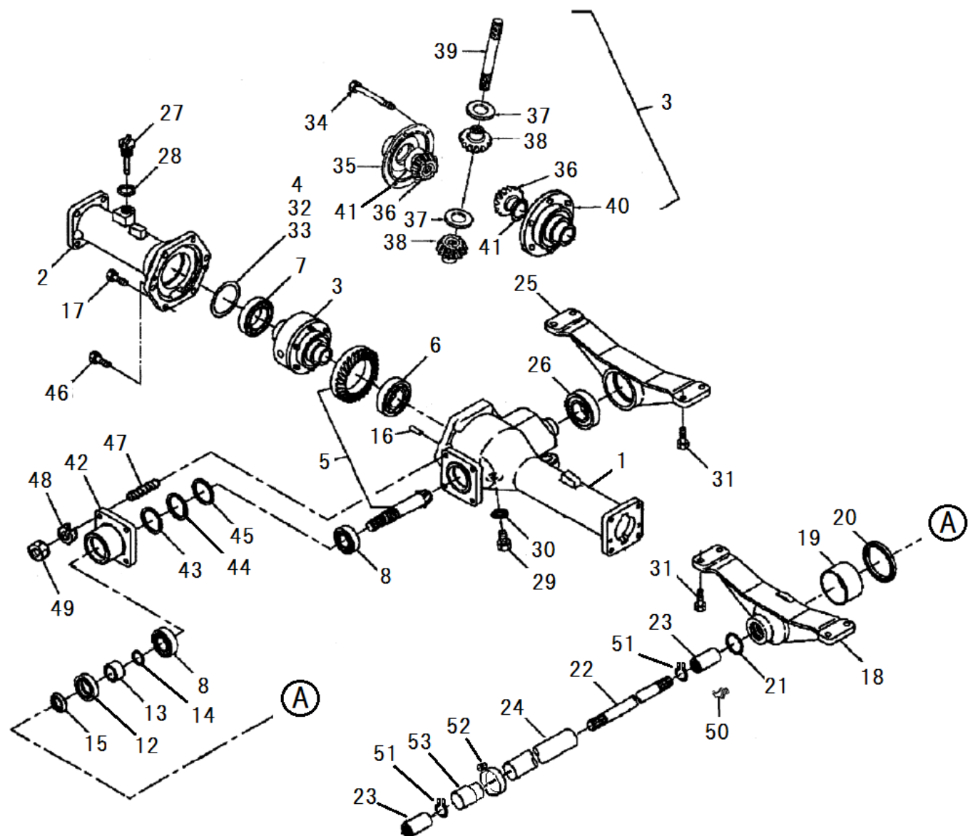
リヤアクスル、デフ&ハウジング FIG.211 REAR AXLE, DIFFERENTIAL & HOUSING
