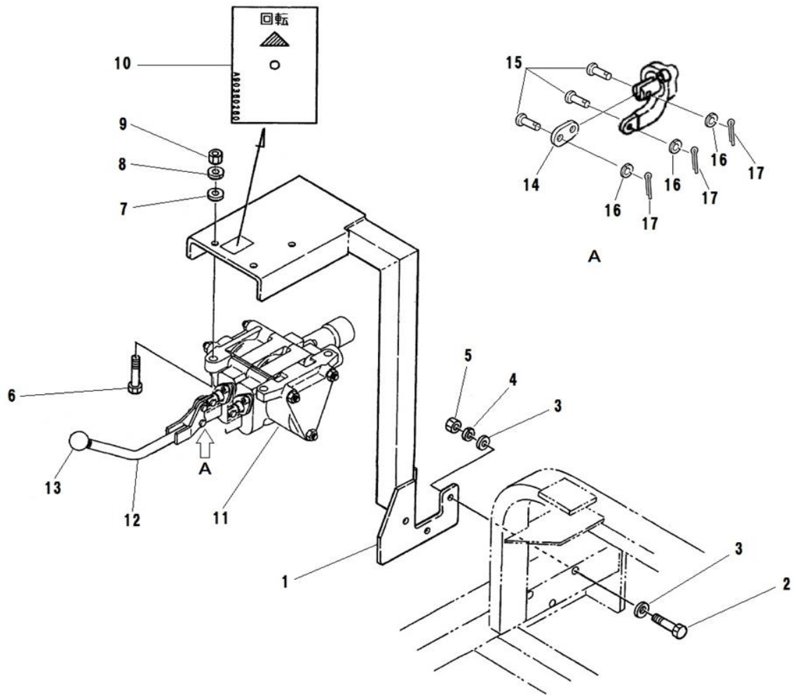
FIG.230 VALVE STAY M バルブステイ M
