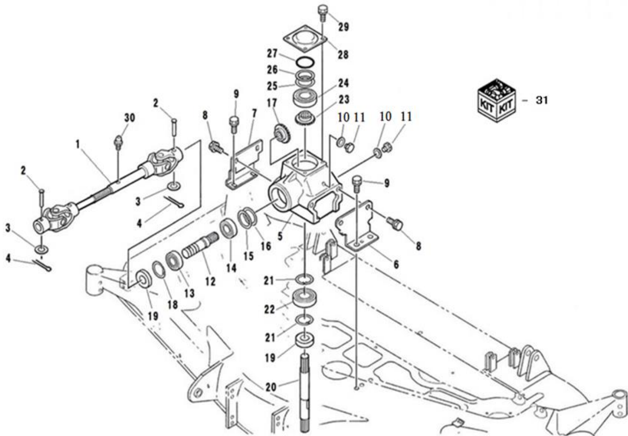
FIG.304 DRIVING クドウ
