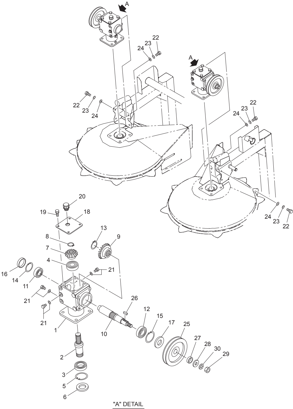
"A" DETAIL
