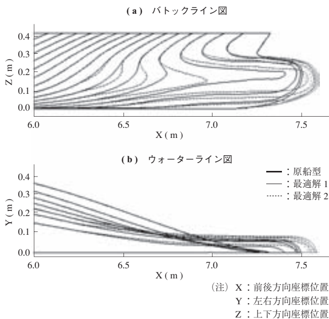
第 8 図 原船型と最適解の船型比較 Fig. 8 Comparison of the initial and optimized hull forms
