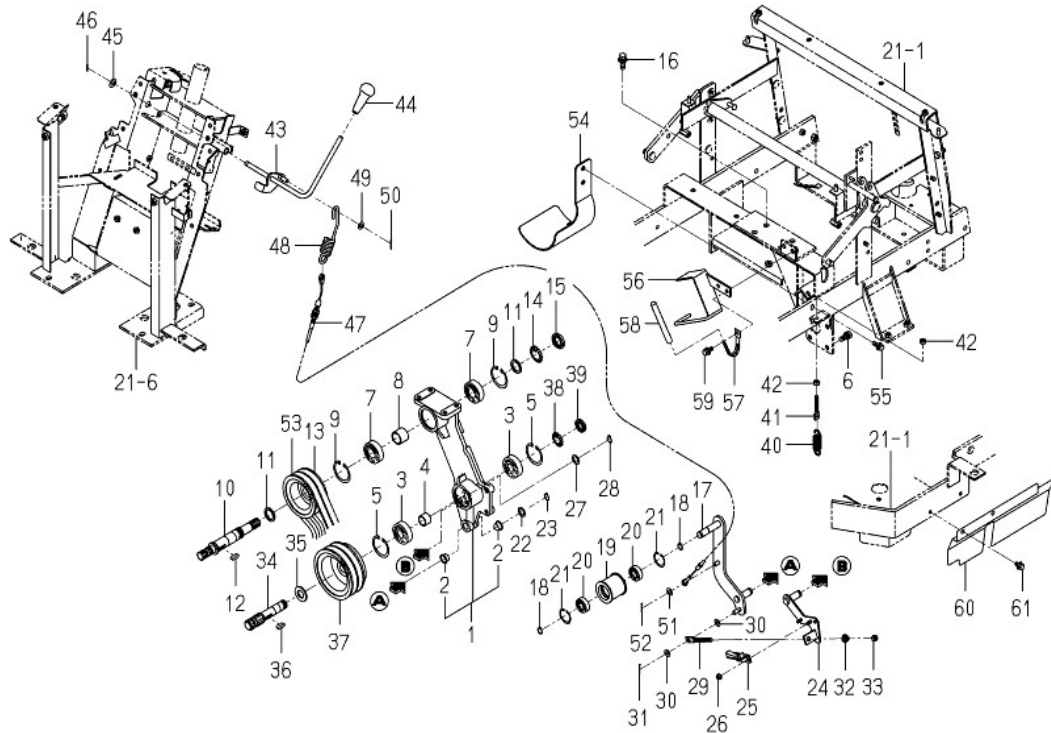
FIG.219 PTO PTO(MOWER)SYSTEM
