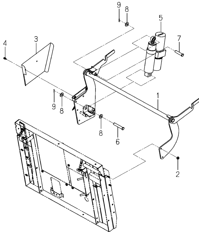
FIG.405 リフト LIFT SYSTEM(A TYPE)
