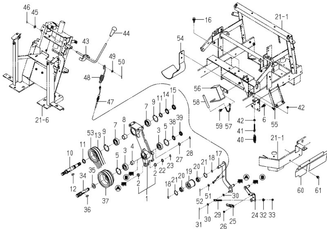
FIG.219 PTO PTO(MOWER)SYSTEM
