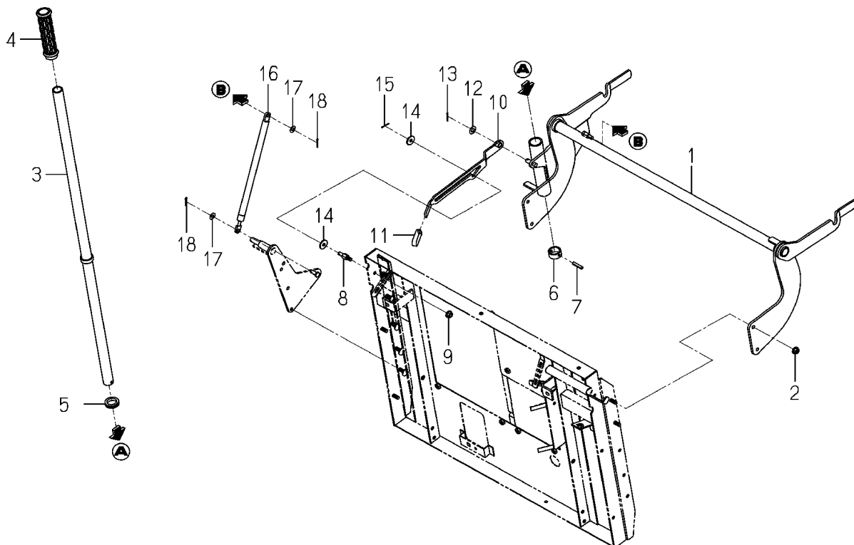
FIG.403 リフト LIFT SYSTEM(EXCEPT A TYPE)
